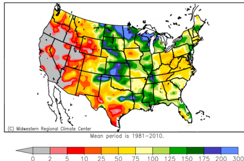
Accumulated Precipitation: Percent of Mean July 1, 2020 to July 21, 2020
